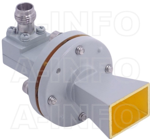
LB-19-15-C-2.4F Standard Gain Horn Antenna 40-50GHz 15dB Gain 2.4mm Female
